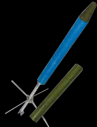
40 mm Round GG-7A IN with Practice Grenade
